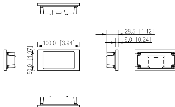
DHI-VTO4103FB-MR.DHI-VTO4103FB-MR1
