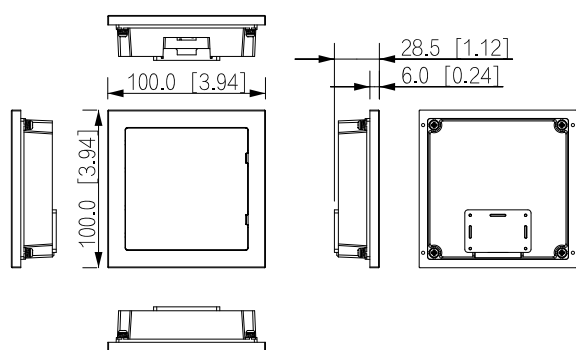
DHI-VTO4103FB-MI
