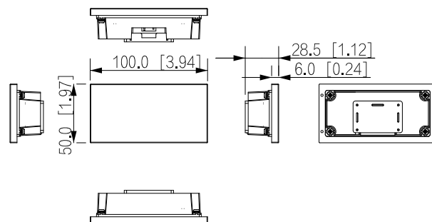
DHI-VTO4103FB-MN
