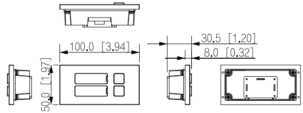
DHI-VTO4103FB-MB1
