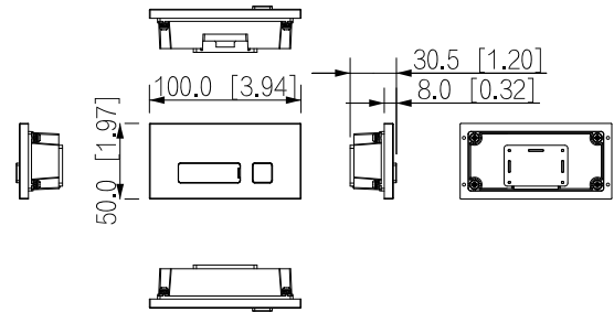
DHI-VTO4103FB-MB1
