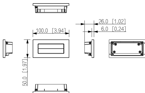
DHI-VTO4103FB-MDB4
