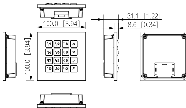
DHI-VTO4103FB-MK
