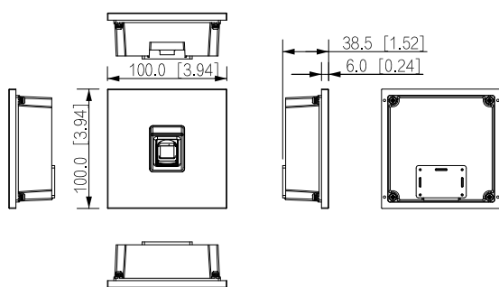
DHI-VTO4103FB-MF
